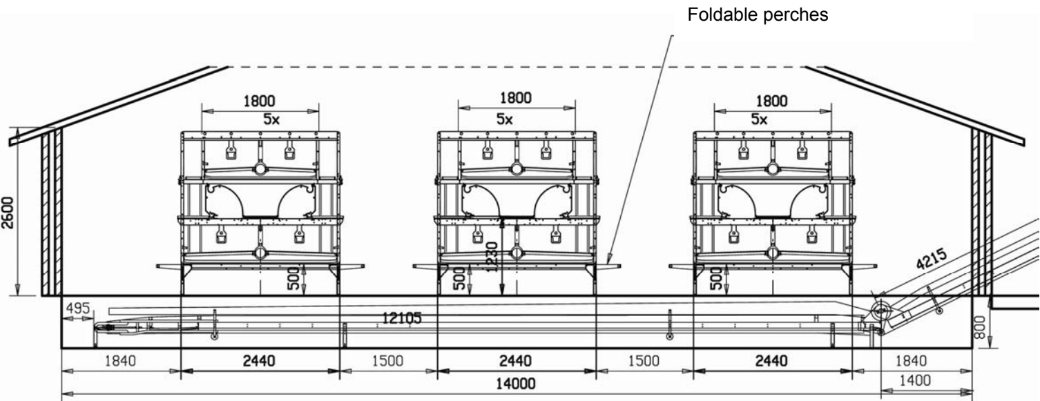
House 75 x 14 for ca. 17.000 leghennen
